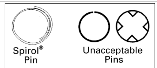
FIGURE 1– Pin Designs
